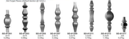
Döme Motifli Parçalar \varnothing 12-14-16mm. Hot Forged Pieces (Default Section: \varnothing 12mm.)
